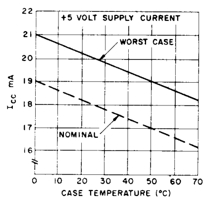
Fig.26 +5 VOLT SUPPLY CURRENT
