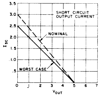
Fig.23 SHORT CIRCUIT OUTPUT CURRENT
